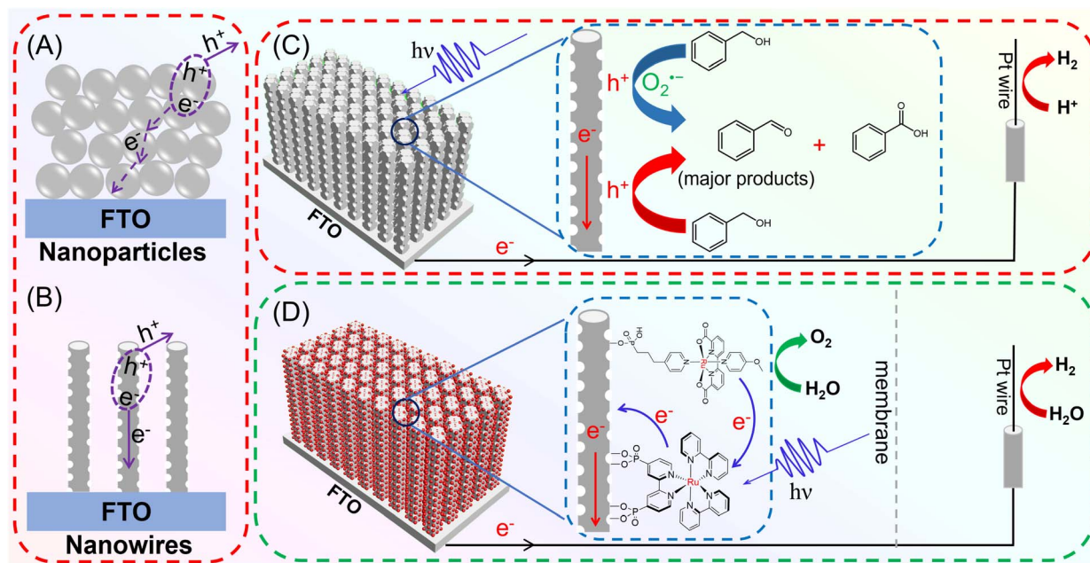
Scheme 1 Schematic illustrating two typical \text{TiO}_2 -based photoelectrodes and their corresponding charge separation/transport behaviors, (A) nanoparticles and (B) nanowires; UCW- \text{TiO}_2 as the photoanode platform for efficient charge separation and collection in photoelectrochemical cells: (C) reaction mechanism for the PEC selective aerobic oxidation of benzyl alcohols from the pristine UCW- \text{TiO}_2 photoanode and simultaneous \text{H}_2 production; (D) Rubda and RuP sensitized UCW- \text{TiO}_2 photoanode assembly and the proposed mechanism of electron transfer and charge collection for water oxidation.
