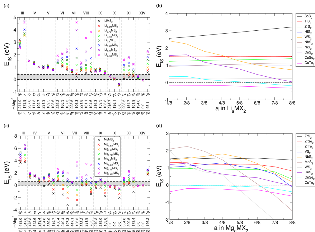
Fig. 8 E_{IS} values for each of the TMDC sulfides intercalated with different concentrations of lithium (a) and magnesium (c). The resultant gravimetric charge capacities in mA\ h\ g^{-1} (as determined from the range over which E_{IS} is positive) are also presented at the bottom of each of (b) and (d) give specific examples of the variation of E_{IS} with lithium and magnesium content, respectively.
