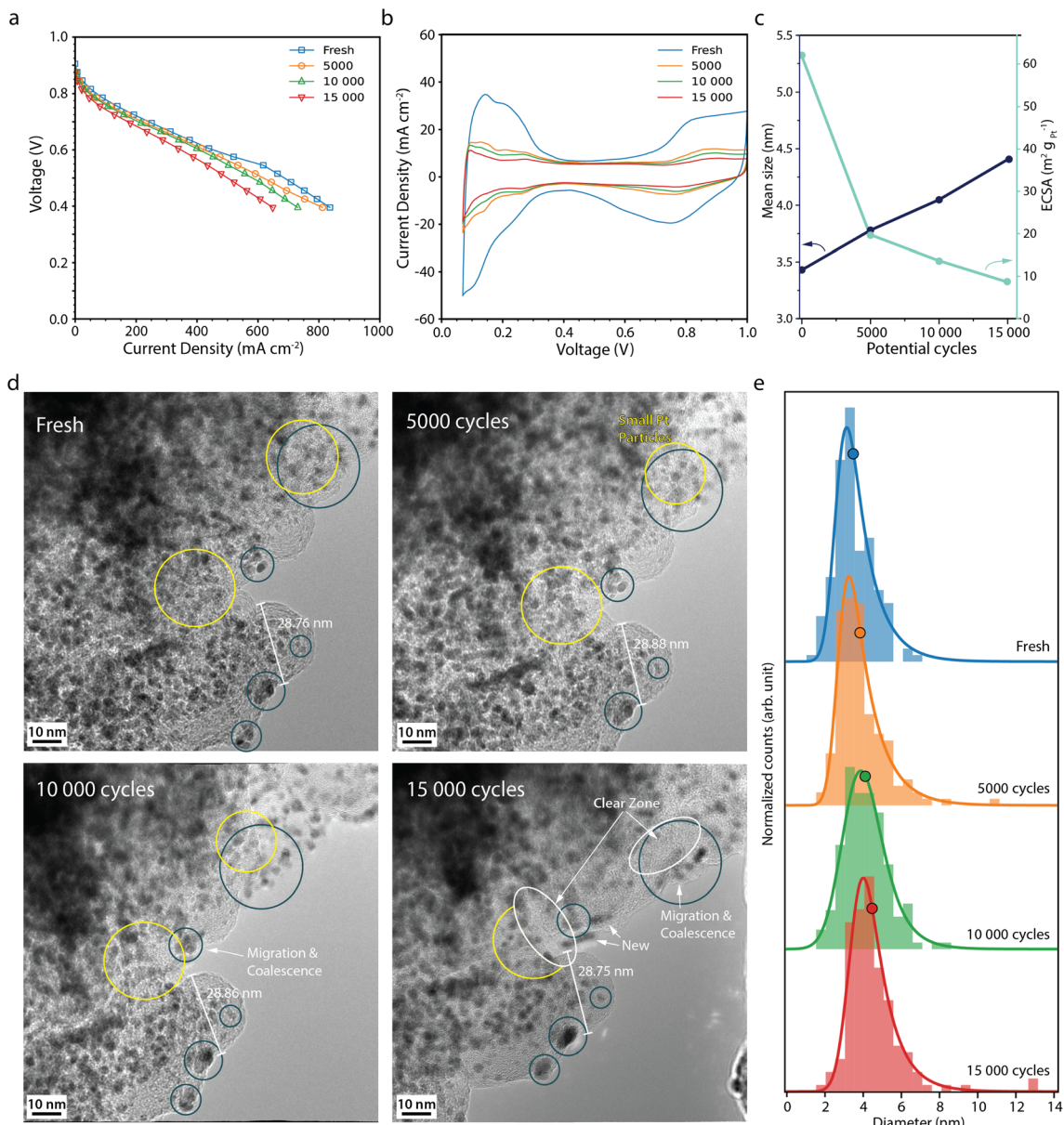
Fig. 2 (a) Polarisation curves measured potentiostatically, and (b) cyclic voltammograms recorded at 100 mV s -1 for the fresh fuel cell and after 5000, 10 000 and 15 000 normal operation AST potential cycles. (c) Mean Pt particle size (black) and available Pt surface area, ECSA, (light blue) versus the number of potential cycles. (d) Corresponding IL-TEM images, and (e) corresponding Pt particle size distributions. The histograms, from 150 Pt particles at each point in time, are fitted with an exponentially modified Gaussian function, and the mean diameter is marked with a circle.
