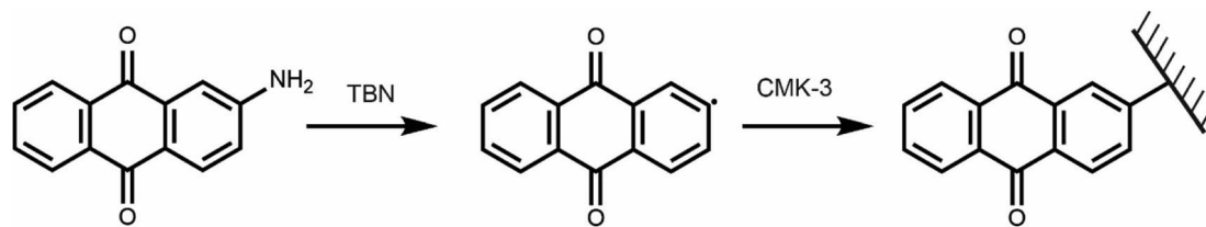
Scheme 2 Functionalisation of CMK-3 using 2-AAQ and tert -butyl nitrite (TBN) used as the radical initiator.
