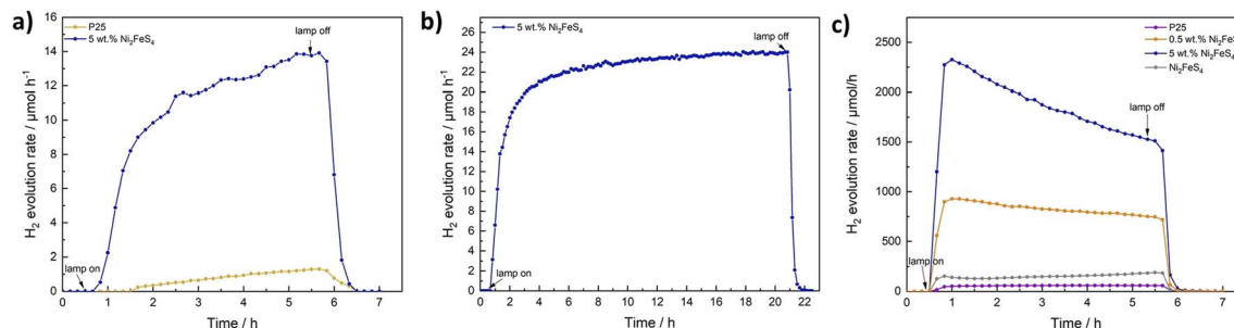
Fig. 8 Photocatalytic HER over P25 and 5 wt% \text{Ni}_2\text{FeS}_4 @P25 using ethanol as a scavenger (a), for longtime irradiation (1 sun) of 5 wt% \text{Ni}_2\text{FeS}_4 @P25 in aqueous methanol solutions (b), as well as HER rates under UV irradiation (c).
