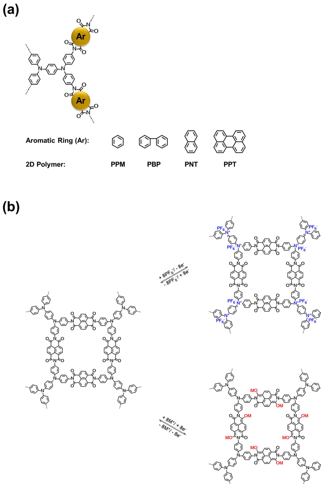
Scheme 1 Structures and reaction mechanism: (a) the molecular structure of four conjugated mesoporous polymers; (b) the proposed reaction mechanism for PNT as an example, where M represents Na/K ion.
