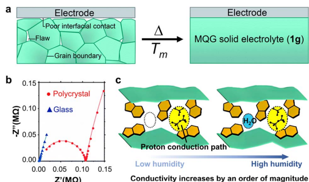
Fig. 5 (a) Melt-quenching of polycrystalline Zn-phosphate-azolate electrolyte into glass eliminated flaws at the electrode–electrolyte interface. (b) The melt-quenched MOF glass electrolyte showed only the bulk impedance response, while the polycrystalline MOF electrolyte showed additional response corresponding to the electrode–electrolyte interface. Adapted with permission from ref. 13, copyright 2021 The Royal Society of Chemistry. (c) Zn-phosphate MOF glass with water uptake ability showed increase in conductivity by an order of magnitude between low and high relative humidity conditions. Adapted with permission from ref. 43, copyright 2019 The Royal Society of Chemistry.
