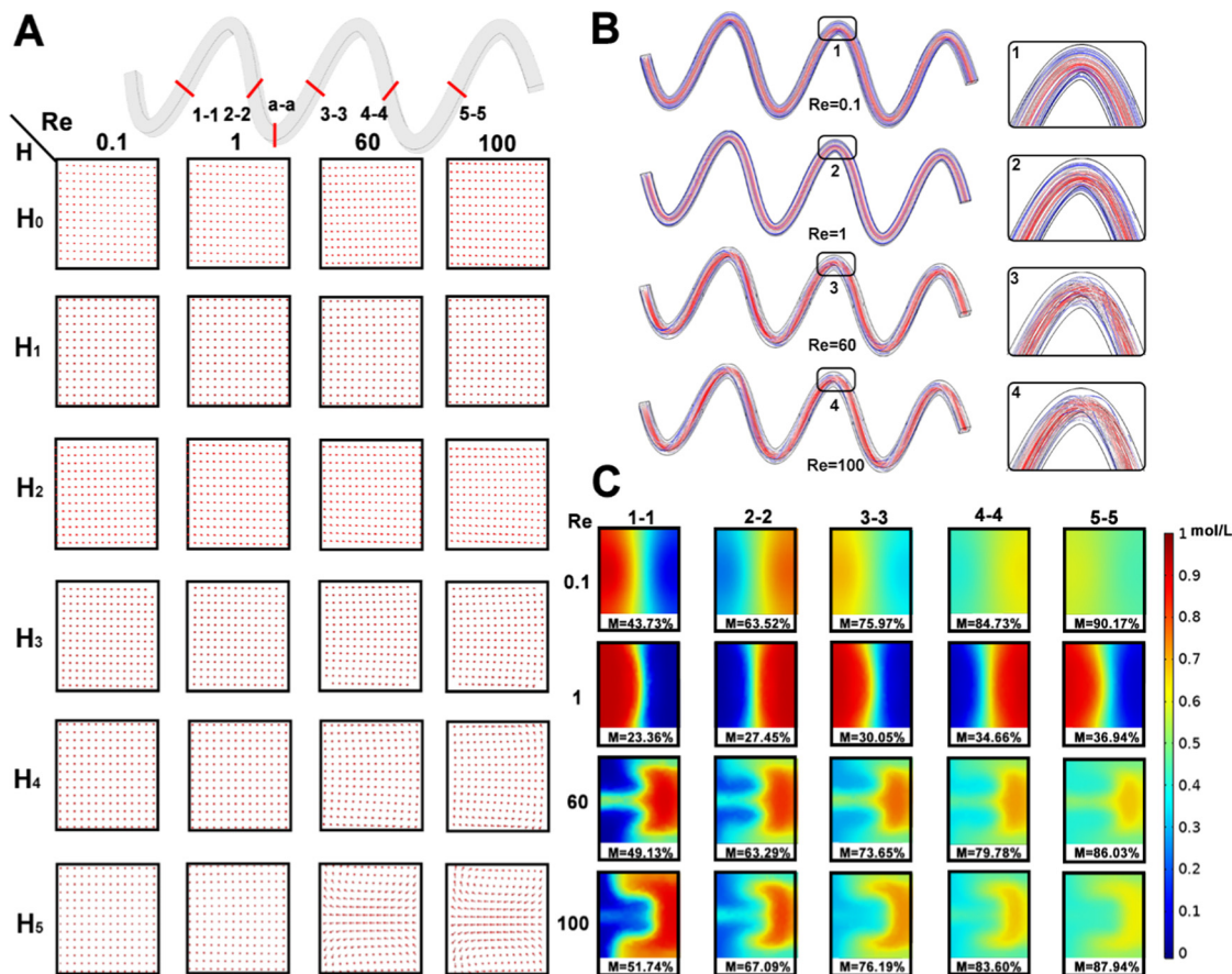
Fig. 4 (A) Flow direction of six hyperbolic curves of the micromixer at different Re for the cross-sections. (B) Streamlining of the hyperbolic micromixer curve H 5 micromixer at different Re and amplified view at channel and curves. (C) Concentration distribution of the cross-section of the hyperbolic curve H 5 of the micromixer at different Re.
