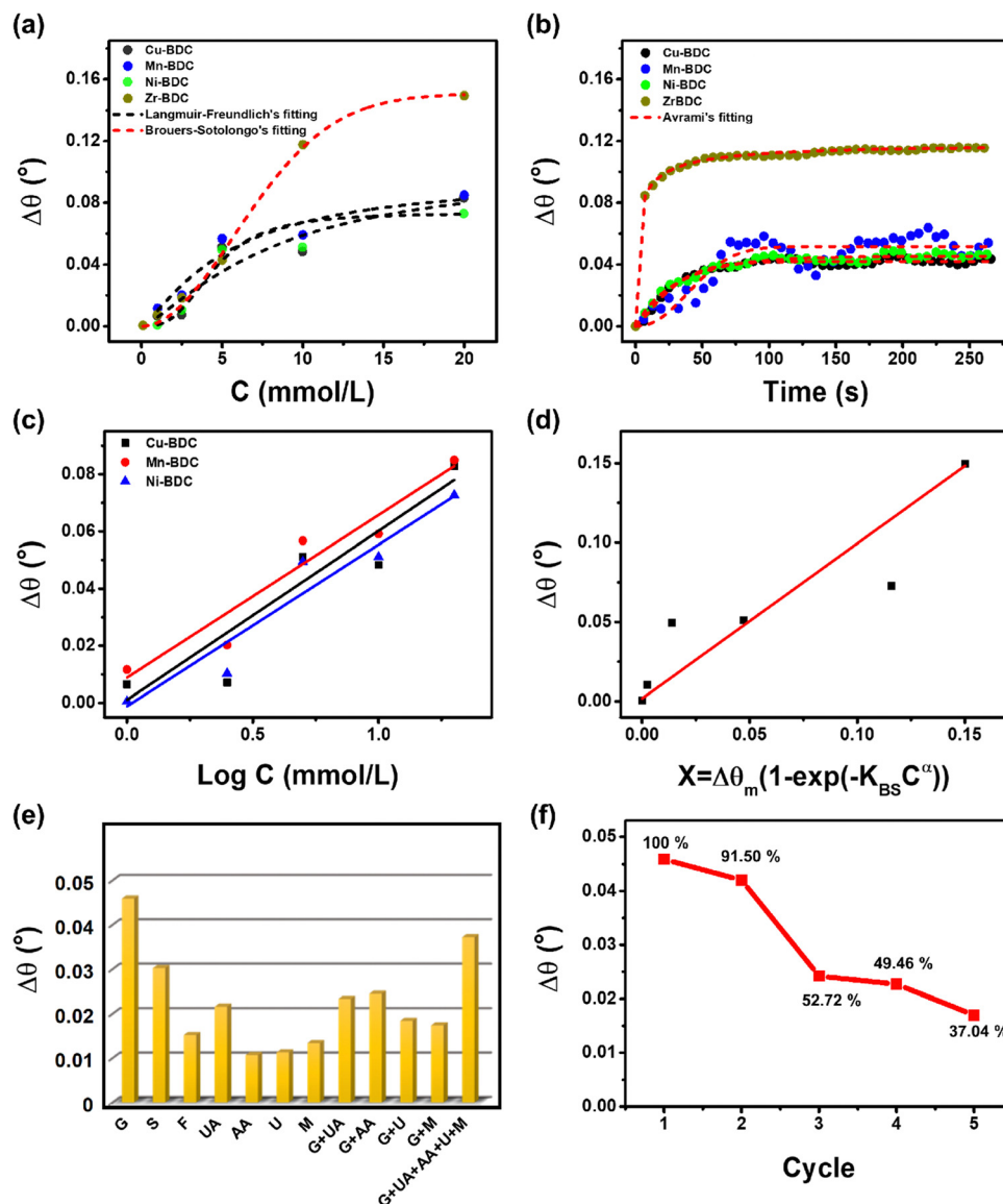
Fig. 4 (a) Non-linear regression curves of Langmuir–Freundlich adsorption isotherm models for glucose-M-BDC ( M = \text{Cu, Mn, and Ni} ) and Brouers–Sotolongo for glucose-Zr-BDC. (b) Non-linear regression curves of the Avrami adsorption kinetic models for glucose-M-BDC ( M = \text{Cu, Mn, Ni, and Zr} ). (c) Calibration curves of the dynamic responses of the M-BDC-functionalized SPR sensors towards glucose: Cu-BDC (black), Mn-BDC (red), and Ni-BDC (blue) are obtained by applying linear fitting to the \Delta\theta vs. \log C plots (Langmuir–Freundlich model), and (d) Zr-BDC is obtained by applying linear fitting to the \Delta\theta vs. X = \Delta\theta_m [1 - \exp(-K_{BS} C^\alpha)] plots (Brouers–Sotolongo model). (e) Bar diagrams showing the angular changes of the Zr-BDC-functionalized SPR sensor upon exposure to various molecules [5 mM glucose (G), 5 mM sucrose (S), and 5 mM fructose (F), 0.45 mM uric acid (UA), 0.11 mM ascorbic acid (AA), 5 mM urea (U), and 0.1 mM maltose (M)]. (f) The corresponding percentage of the dynamic response of Zr-BDC-functionalized SPR sensor to 5 mmol L -1 glucose after the n th measurement compared to the first measurement.
