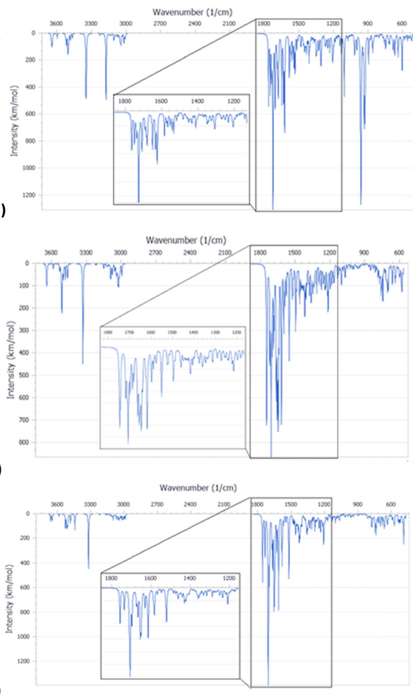
Fig. 9 IR spectra simulated from the calculated molecular structure with DFT for PNA tetramer 1 (chloride salt) (a), PNA tetramer 2 (Na salt) (b), and PNA tetramer 3 (c).
