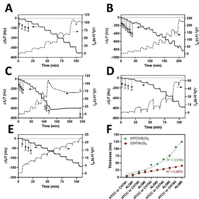
Fig. 5 QCM-D monitoring of the normalized frequency ( \Delta f/7 ) and dissipation ( \Delta D/7 ) shifts at the 7 th overtone as a function of time for the build-up of (A) (HTCC/ALG) 5 , (B) (HTCC/ALG/HTCC/FITC-BSA) 5 and (C) (HTCC/ALG) 5 /HTCC/FITC-BSA multilayered thin films in 10 mM PBS at pH 7.4, and (D) (HTCC/ALG) 5 and (E) (CHT/ALG) 5 in 0.1 M acetate buffer at pH 5.5, onto Au-coated quartz crystal sensors. The inset numbers in: (A) and (D) refer to the adsorption of HTCC (1), ALG (3), and rising steps (2 and 4); (B) and (C) refer to the adsorption of HTCC (1 and 5), ALG (3), FITC-BSA (7) and rising steps (2, 4, 6 and 8); (E) refer to the adsorption of CHT (1), ALG (3), and rinsing steps (2 and 4). (F) Cumulative hydrodynamic thickness evolution for the (HTCC/ALG) 5 and (CHT/ALG) 5 films as a function of the number of deposited layers, estimated using the Voigt-based viscoelastic model. The red and green lines represent the linear and exponential trend lines, respectively.
