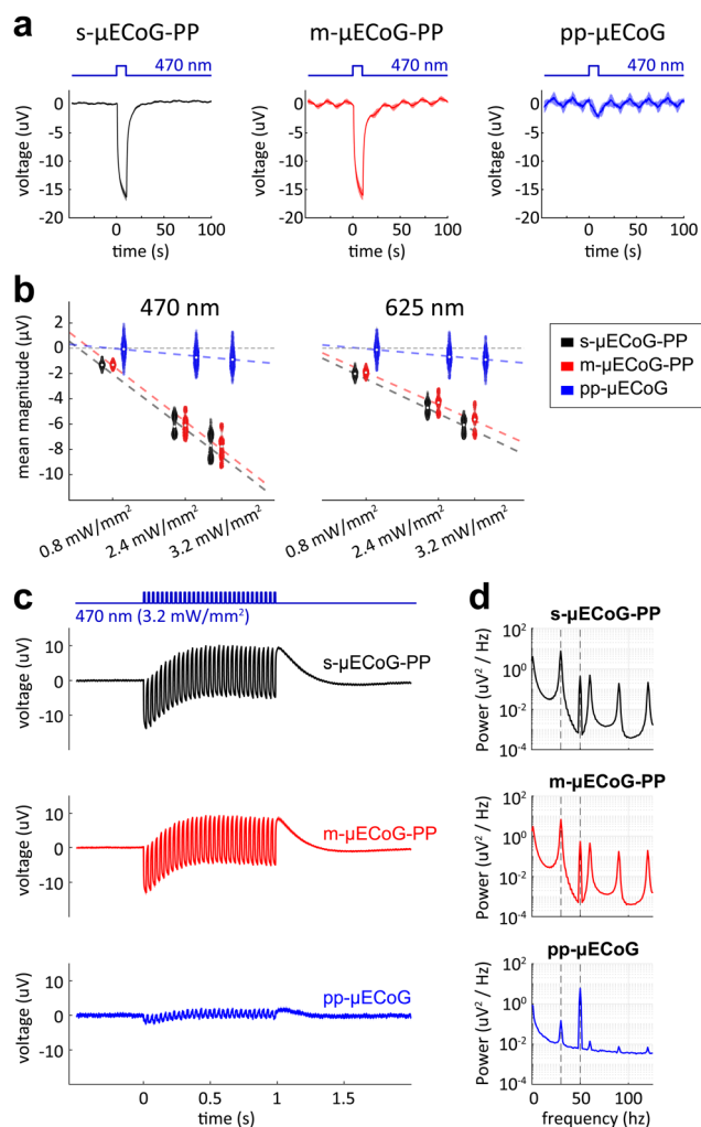
Fig. 4 Characterization of light-induced artefacts in saline solution. Recording of light-induced artefacts from s-, m-, and pp- \mu ECoG electrodes, in response to a 10-ms long light pulse ( \lambda = 470 \text{ nm} , irradiance = 3.2 \text{ mW mm}^{-2} ) in PBS. Average signals over 125 light pulses on 6 electrodes ( N = 750 in total). (b) Mean magnitude of measured signals for s-, m-, and pp- \mu ECoG electrodes in response to 10 ms long light pulse at different wavelengths ( \lambda = 470 and \lambda = 625 \text{ nm} ) and different light power levels ( N = 750 pulses per condition). Coloured dashed lines show linear regression line for each \mu ECoG type. (c) Recording of light-induced artefacts from s-, m-, and pp- \mu ECoG electrodes, in response to a 1 s long, 30 Hz stimulation sequence, as commonly used during functional imaging. Traces show average signals over 20 light sequences on 6 electrodes ( N = 120 in total). (d) Power spectral density for each \mu ECoG type during 30 Hz stimulation as shown in (c). Grey dashed lines indicate light-induced oscillations at 30 Hz and line noise at 50 Hz.
