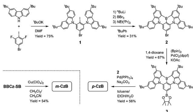
Scheme 1 Synthetic Routes to p-CzB and m-CzB .
