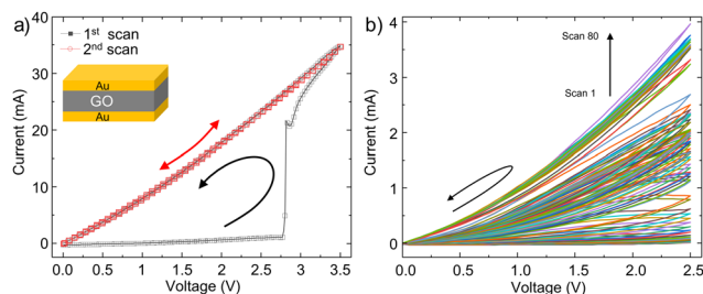
Fig. 1 (a) Current–voltage characteristics of GO crossbar devices (scan rate of 100\text{ mV s}^{-1} ). (b) The evolution of the current–voltage characteristics of a GO device after 80 consecutive scans with a scan rate of 100\text{ mV s}^{-1} . The arrows indicate the direction of the current hysteresis.
