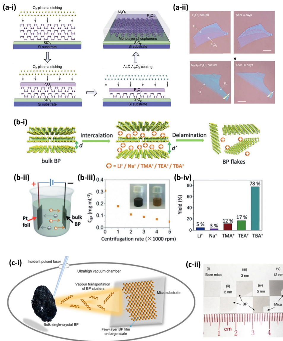
Fig. 8 (a) Mechanically exfoliated black phosphorus (BP) on a \text{SiO}_2/\text{Si} substrate treated with \text{O}_2 plasma etching: (a-i) schematic illustration of the preparation process, and (a-ii) OM images of single-layer BP covered by \text{P}_2\text{O}_5 or \text{P}_2\text{O}_5/\text{Al}_2\text{O}_3 capping layer before and after several days. 109 Reproduced with permission from ref. 109. Copyright 2016, Springer Nature. (b): Electrochemically exfoliated BP: (b-i) Schematic delamination procedure, (b-ii) Experimental setup, (b-iii) Concentration of BP as a function of centrifugation rate, and (b-iv) Delamination yield as a function of intercalating cations. 125 Reproduced with permission from ref. 125. Copyright 2016, John Wiley-VCH.
