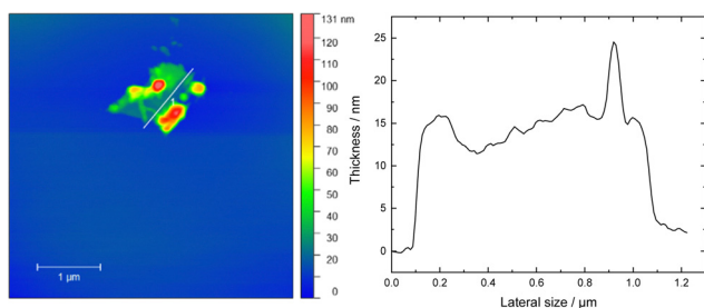
Fig. 4 AFM image and the corresponding height profile plot of exfoliated \text{NiGa}_2\text{S}_4 .
