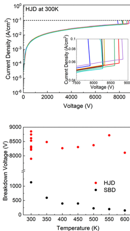
Fig. 4 (top) Spread of reverse current characteristics from NiO/Ga 2 O 3 heterojunction rectifiers at 300 K. (bottom) Temperature dependence of breakdown voltage for Schottky barrier diodes and heterojunction diodes.
