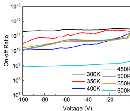
Fig. 7 On-off ratio of (top) Schottky rectifiers and (bottom) \text{NiO}/\text{Ga}_2\text{O}_3 heterojunction rectifiers in which the bias was switched from 5 V forward to the voltage shown on the x-axis.
