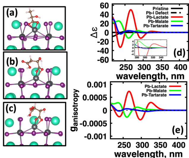
Fig. 6 Conformers bonded to excess \text{Pb}^{2+} on the \text{CsPbI}_3 cluster surface with the largest Boltzmann weights for (a) (S)-lactate, (b) (S)-malate, and (c) (S,S)-tartarate. The color scheme for atomistic structures correspond to Cs (teal), Pb (grey), I (purple), O (red), C (brown), and H (white). (d) CD and (e) anisotropy spectra for the pristine \text{CsPbI}_3 cluster (black, solid), cluster with excess \text{Pb}^{2+} surface defect (black, dash-dot), (S)-lactate (red), (S)-malate (green), and (S,S)-tartarate (blue) bonded to the surface \text{Pb}^{2+} site. The panel (d) inset shows the spectra near the optical gap. In panel (e), the black dashed line represents the zero level for reference.
