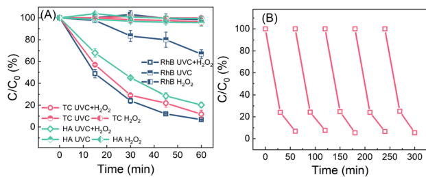
Fig. 4 (A) The removal of RhB, TC and HA via UVC/H 2 O 2 , UVC and H 2 O 2 processes in batch tests; and (B) recyclability of the process for RhB removal (RhB, TC or HA: 1 mg L -1 ; H 2 O 2 : 10 μM).
