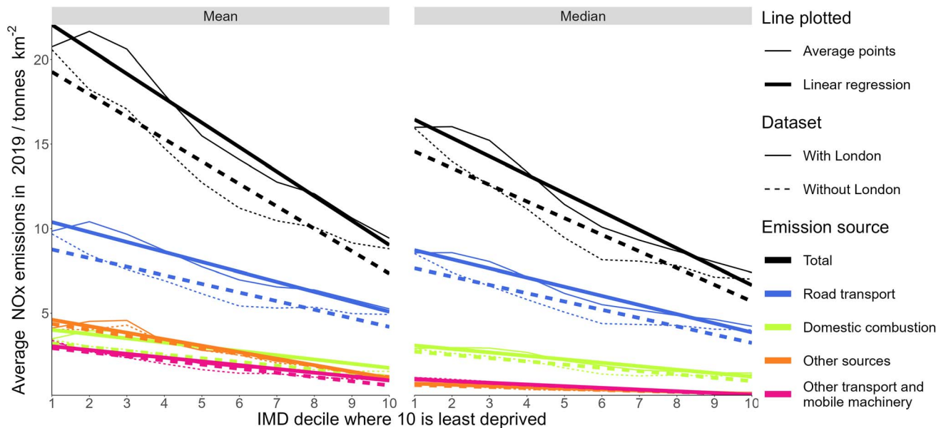
Fig. 2 The mean and median emissions of NO x , by LSOA across England for major source sectors, the average without London is also shown. The category "Other sources" is the combination of the source sectors: agricultural; energy production; industrial combustion; industrial combustion; solvents; natural; and point sources.
