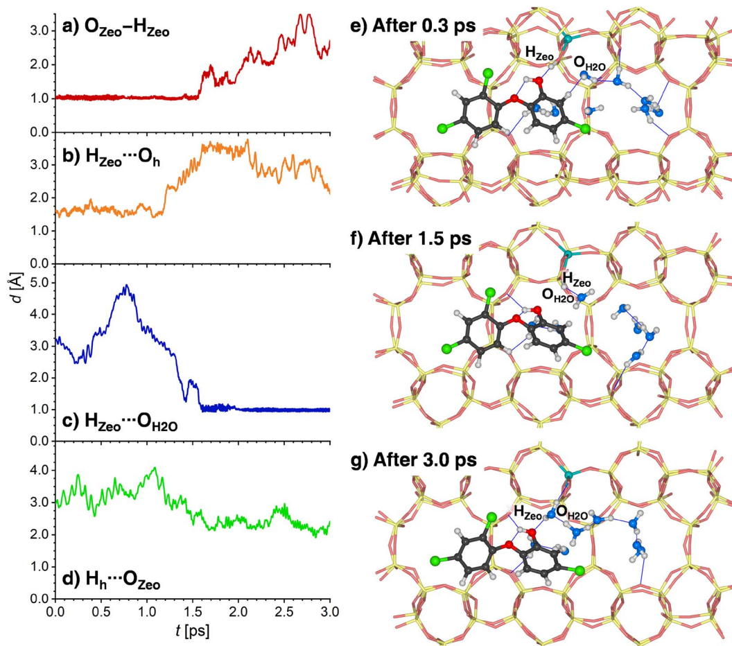
Fig. 9 (a)–(d) Evolution of selected interatomic distances during the first 3 ps of one AIMD trajectory (Traj1) computed for 8H 2 O@(TCS@H-MOR), (e)–(g) environment of the framework Al atom at different stages of the simulation.
