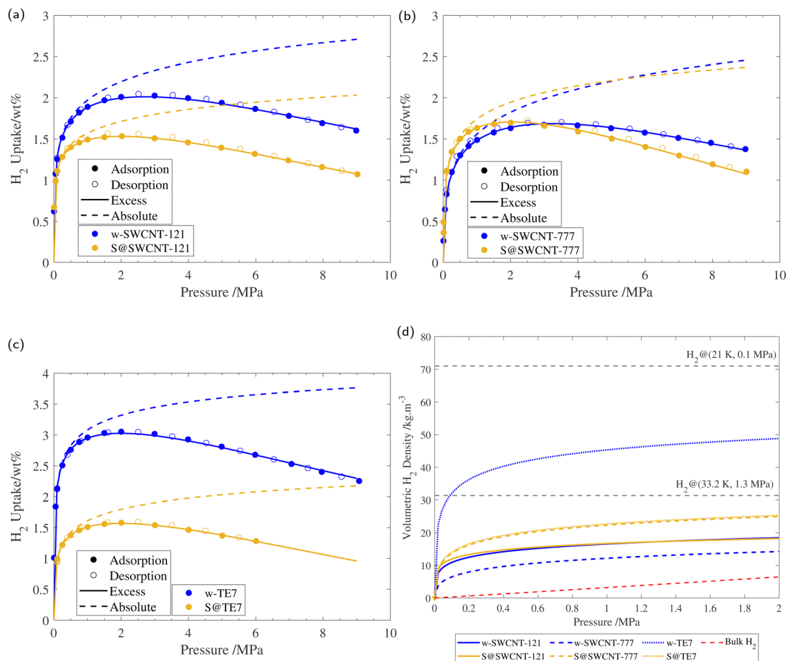
Fig. 5 (a) 77 K H 2 sorption isotherm of w-SWCNT-121 and S@SWCNT-121, with the respective excess isotherm determined through fitting and absolute isotherm, calculated using eqn (3). (b) 77 K H 2 sorption isotherm of w-SWCNT-777 and S@SWCNT-777, with the respective excess isotherm determined through fitting and absolute isotherm, calculated using eqn (3). (c) 77 K H 2 sorption isotherm of w-TE7 and S@TE7, with the respective excess isotherm determined through fitting and absolute isotherm, calculated using eqn (3). (d) Volumetric hydrogen density versus pressure up to 2 MPa for w-SWCNT-121 (blue solid line), S@SWCNT-121 (yellow solid line), w-SWCNT-777 (blue dashed line), S@SWCNT-777 (yellow dashed line) and S@TE7 (yellow dotted line), calculated using eqn (4). NIST bulk hydrogen data at 77 K (red dashed line), Liquid hydrogen density (20.25 K, 0.1 MPa), and density of hydrogen at its critical point (33.20 K, 1.3 MPa) are shown for reference. Each isotherm shows the result of the 3rd repeat run, all isotherms can be found in the ESI† (see Fig. S8).
