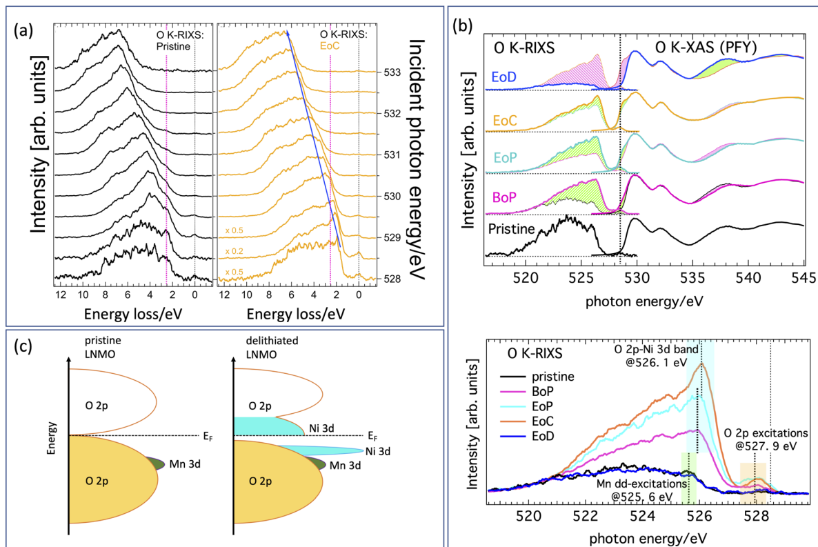
Fig. 3 (a) Waterfall plots for O K-edge RIXS of pristine (left panel) and fully delithiated LNMO (right panel). The spectra are normalized to unit height. The magenta vertical dashed lines mark mediated Mn dd-excitations at a fixed energy loss of approximately 2.5 eV and the blue arrow in right panel highlights the fluorescence-like dispersion of the O 2p–Ni 3d band feature. (b) Top panel: O K-edge RIXS and XAS spectra at different SoC. Light green (pink) shading indicates increment (decrement) of intensity compared to the previous SoC. The long vertical dashed line marks the incident photon energy (at 528.5 eV) of the RIXS spectra. Bottom panel: Overlaid O K-edge RIXS spectra showing their natural intensity variation relative to each other. The color-shaded rectangles indicate various energy regions of interest: intra band O 2p excitations (orange), Mn dd-excitations (green), O 2p–Ni 3d-hybridization band (turquoise). (c) Energy diagram derived from the RIXS and XAS spectra illustrating the effects of delithiation on the oxygen states by re-hybridization with nickel states.
