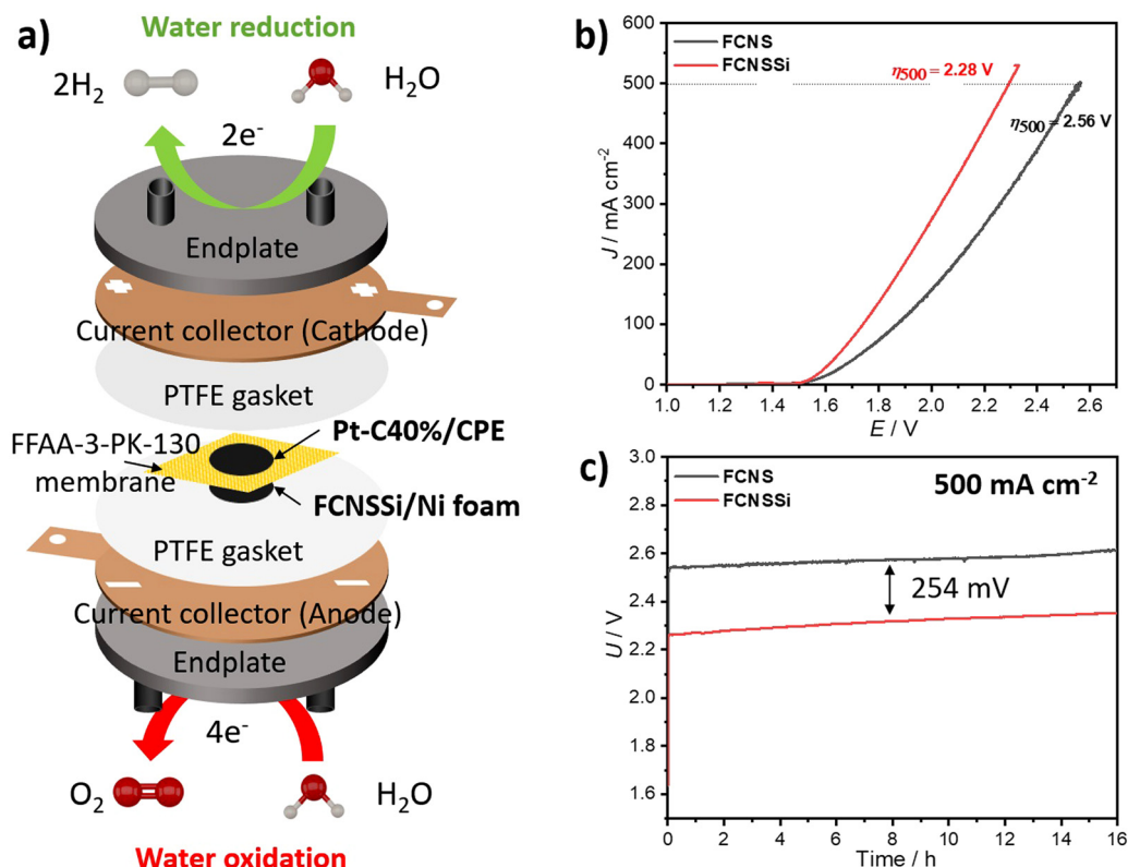
Fig. 9 (a) Zero-gap cell assembly using FCN/SSi on Ni foam at anodic side against Pt/C (40%) on CPE at cathodic side, and (b) LSV measurements, and (c) chronopotentiometry test at 500 \text{ mA cm}^{-2} for 16 h of both pristine FCNS and FCN/SSi on Ni foam electrodes.
