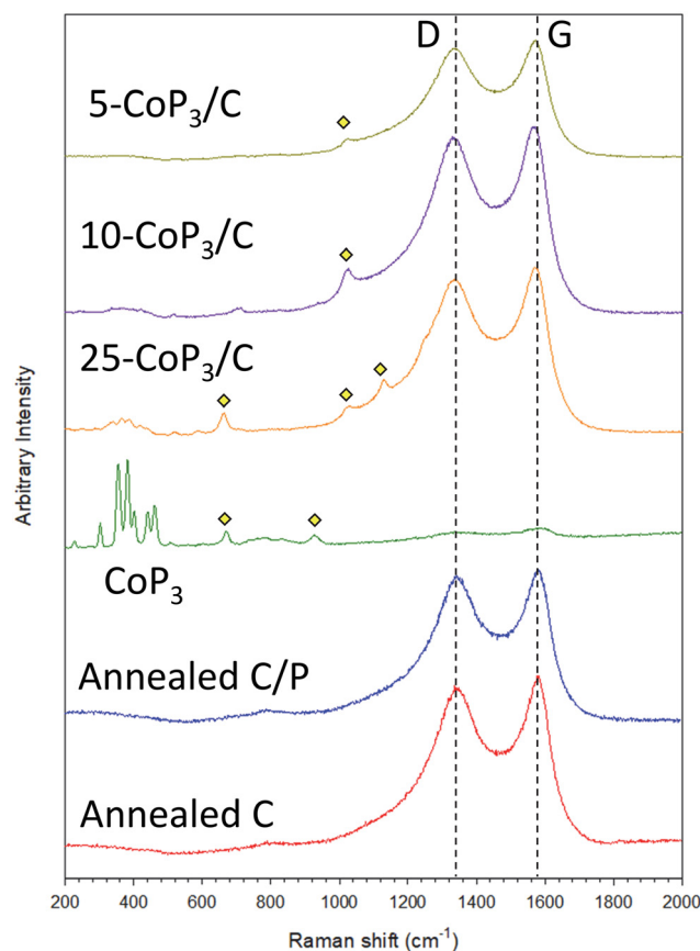
Fig. 3 An overlay of Raman spectra of \text{CoP}_3 , x\text{-CoP}_3/\text{C} ( x = 5, 10, 25 ) and 500 °C annealed carbon black alone (C) and carbon black annealed with phosphorus (C/P) in the region of 200–2000 cm -1 . (◆) denotes peaks for P–O bonding.
