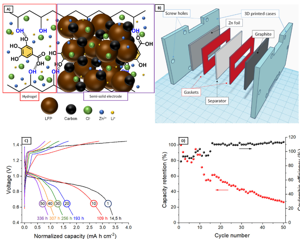
Fig. 5 (A) Scheme of the semi-solid electrode composition. (B) Schematic representation of the simple-shape battery. (C) Voltage profiles for the Zn|G1|G1-KB+LFP|graphite simple-shape battery ( L \times W \times H = 5 \times 1 \times 0.1 \text{ cm}^3 ) operated at 0.5 \text{ mA cm}^{-2} . A specific capacity of 184 \text{ mA h g}^{-1} was obtained for the 1st cycle. (D) Evolution of the charge capacity and coulombic efficiency with the number of cycles. Total cycling time was 336 h.
