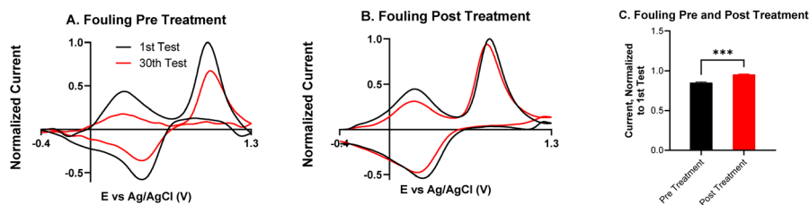
Fig. 7 Electrode fouling measurements at an untreated and a KOH treated CNTYME. 1 \mu\text{M} 5-HT was injected for 5 seconds every 30 seconds, repeated 30 times. (A) CVs from an untreated CNTYME show a decrease on the 30th injection. (B) CVs from a 1-minute KOH treated CNTYME show the signal is largely preserved on the 30th injection. (C) Unpaired t -tests compare the 1st and 30th signal ( p < 0.001 , n = 4 ) and there was a significant difference in the fouling.
