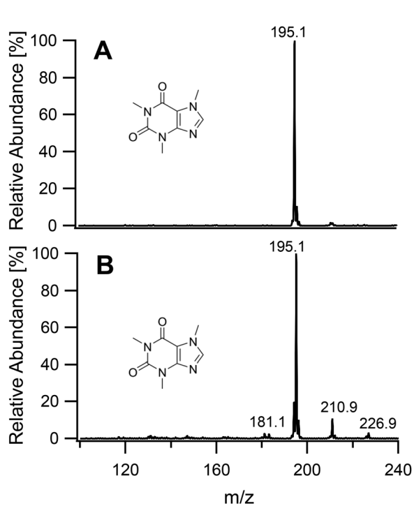
Fig. 6 Mass spectra of caffeine acquired under soft conditions (A) and under fragmenting conditions (B).
