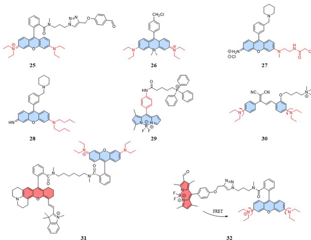
Fig. 8 Structures of intramolecular-rotation-based temperature probes.
