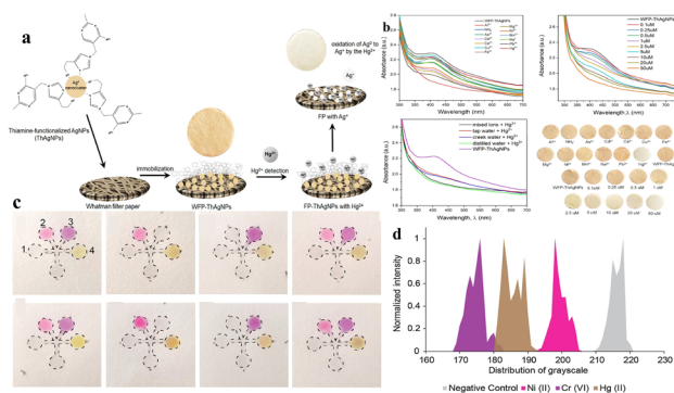
Fig. 2 (a) A schematic representation of the possible mechanism involved in the detection of Hg 2+ through a color change using ThAgNPs anchored on filter paper. (b) UV-vis spectra of WFP–ThAgNPs exposed to different ions and various concentrations of Hg 2+ (reproduced from Budlyan et al. , 2022, Environmental Nanotechnology, Monitoring and Management ). 57 (c) μPAD showing the color development after the application of DI water, 5 ppm of Ni 2+ , Cr 6+ , or Hg 2+ , and heavy metal ion spiked lake-water samples. (d) Graphical representation of the distribution of grayscale vs. normalized intensity (reproduced from Devadhasan and Kim, 2018, with permission from Elsevier). 54
