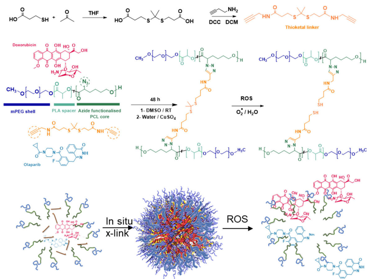
Fig. 6 Synthetic scheme for the preparation of ROS-responsive nanoparticles. A bis(alkynyl) thioketal cross-linker is reacted with mPEG-poly(lactide- co -poly(azido-caprolactone)) in the presence of DOX and OLA to form drug-loaded nanoparticles designed to release payload in the presence of reactive oxygen species (ROS).
