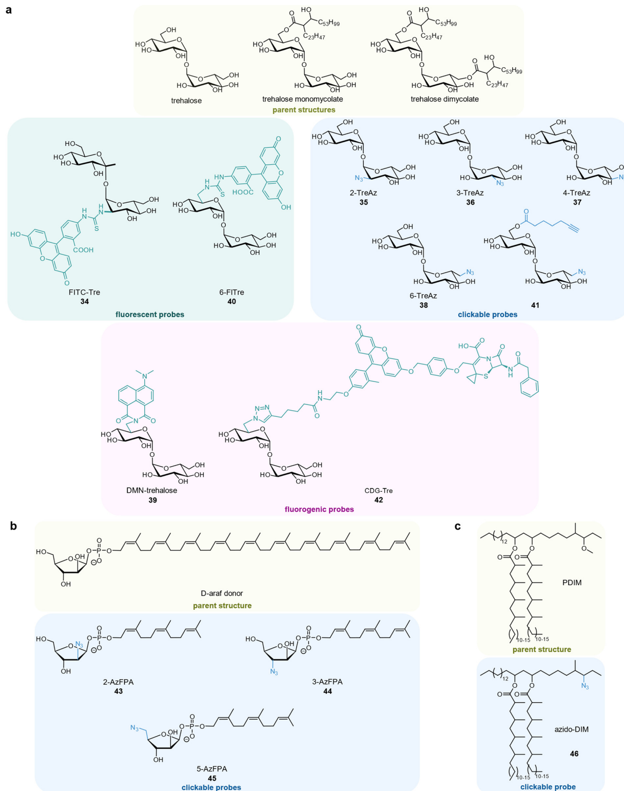
Fig. 6 Mycomembrane components and corresponding probe derivatives. (a) Trehalose-based probes. (b) Arabinose-based probes. (c) Phthiocerol dimycoerolate-based probe.
