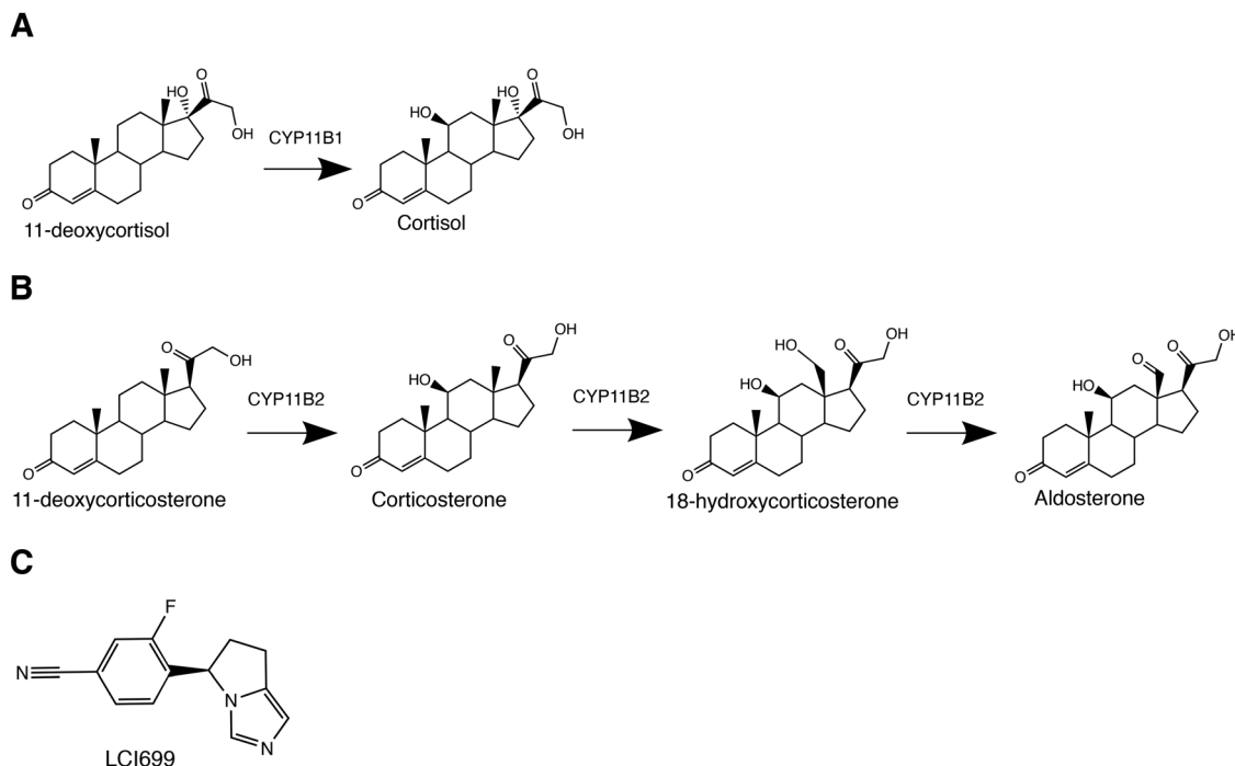
Fig. 1 Cytochrome P450 11B enzyme ligands. (A) The CYP11B1-mediated 11\beta -hydroxylation of 11-deoxycortisol results in the major glucocorticoid hormone cortisol. (B) Human CYP11B2 generates the major mineralocorticoid hormone aldosterone. Similar to CYP11B1, CYP11B2 performs an 11\beta hydroxylation to convert 11-deoxycorticosterone to corticosterone, but subsequently performs an 18-hydroxylation and 18-oxidase reaction to generate aldosterone. (C) LCI699 is an FDA-approved cushing syndrome drug displaying low nanomolar affinity for both CYP11B1 and CYP11B2 and serves as a heme iron-ligating inhibitor.
