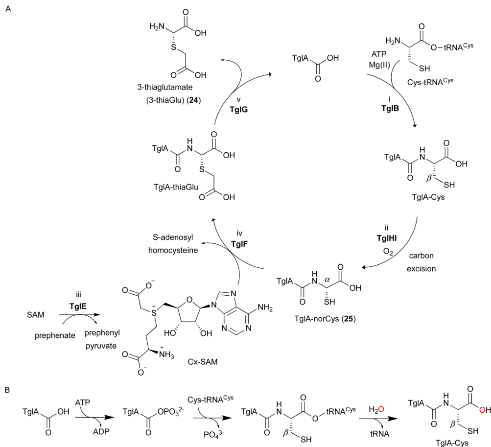
Fig. 12 Biosynthetic pathway of 3-thiaglutamate ( 24 ). (A) 3-thiaglutamate ( 24 ) formation catalyzed by Tgl enzymes. (B) Cysteine addition by the PEARL TgB to the leader peptide TgIA. The reaction starts with phosphorylation of the C-terminal carboxylate of TgIA, which then forms an amide bond with the amino group of Cys-tRNA Cys , followed by the hydrolysis of the tRNA to generate TgIA-Cys. 5
