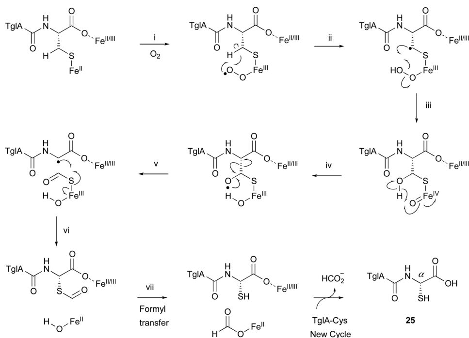
Fig. 13 Proposed mechanism of the TgHI reaction.
