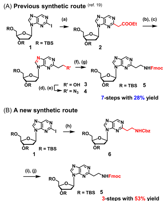
Scheme 1 Optimization of the synthetic route of guanidino-dN. (A) Previous synthetic route, reagents and conditions: (a) \text{Pd}(\text{OAc})_2 , Xantphos, \text{Cs}_2\text{CO}_3 , diethyl malonate, 135^\circ\text{C} , 87%, (b) \text{LiAlH}_4 , THF, -78^\circ\text{C} to 0^\circ\text{C} , (c) DDQ, DCM, r.t., 66% in 2 steps, (d) \text{PPh}_3 , \text{CBr}_4 , DCM, 0^\circ\text{C} to r.t., (e) \text{NaN}_3 , DMSO, r.t., 80% in 2 steps, (f) \text{H}_2 , 10% Pd/C, TEA, MeOH, r.t., (g) FmocCl, TEA, DCM, r.t., 69% in 2 steps. (B) A new synthetic route, reagents, and conditions: (h) benzyl- N -vinylcarbamate, 9-BBN, \text{PdCl}_2(\text{dppe}) , NaOH aq., THF, 65^\circ\text{C} , 65%, (i) \text{Pd}(\text{OH})_2/\text{C} , \text{H}_2 , MeOH, r.t., (j) FmocCl, TEA, DCM, r.t., 82% in 2 steps.
