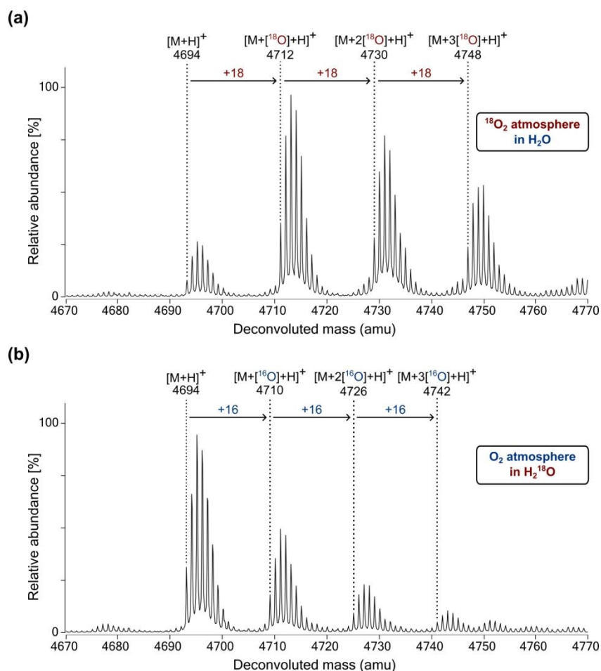
Figure 5. The newly incorporated oxygen atoms in hydroxylated BRD4 511-550 originate predominantly from atmospheric \text{O}_2 .
