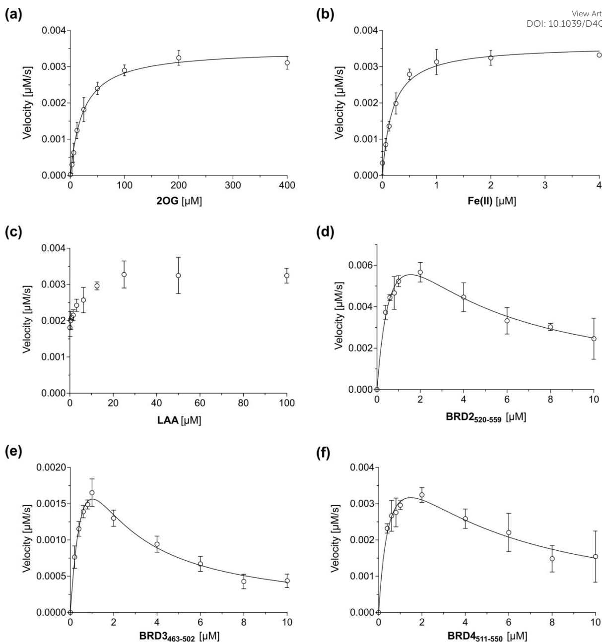
Figure 3. Michaelis-Menten plots used to determine steady-state kinetic parameters for JMJD6.
