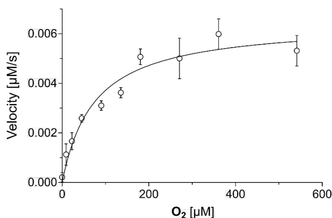
Figure 4. Michaelis-Menten plot used to determine the steady-state kinetic parameters of JMJD6 for O 2 .
