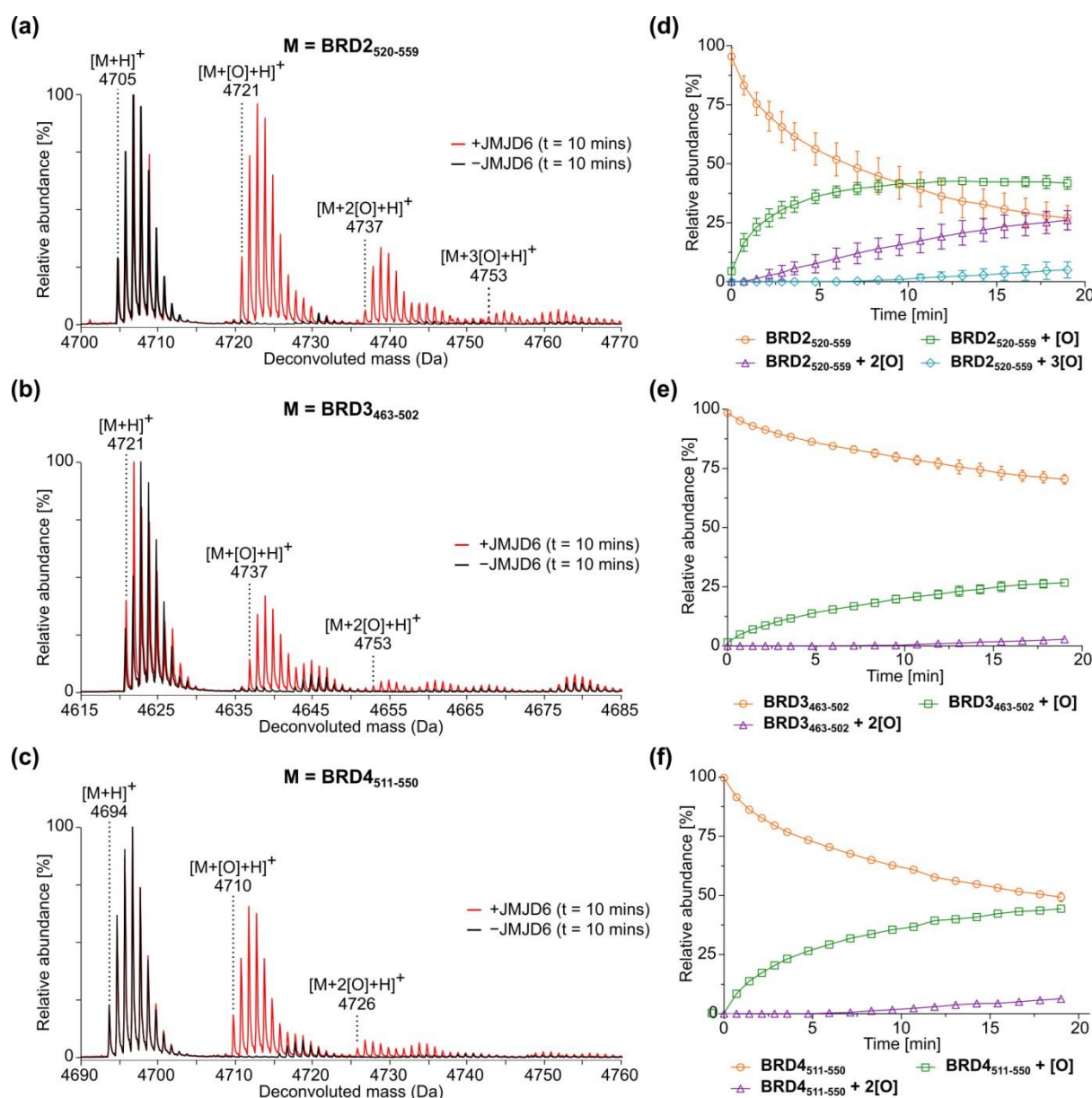
Figure 2. JMJD6-catalysed hydroxylation of homologous 40mer peptides derived from bromodomain-containing proteins BRD2, BRD3, and BRD4.
