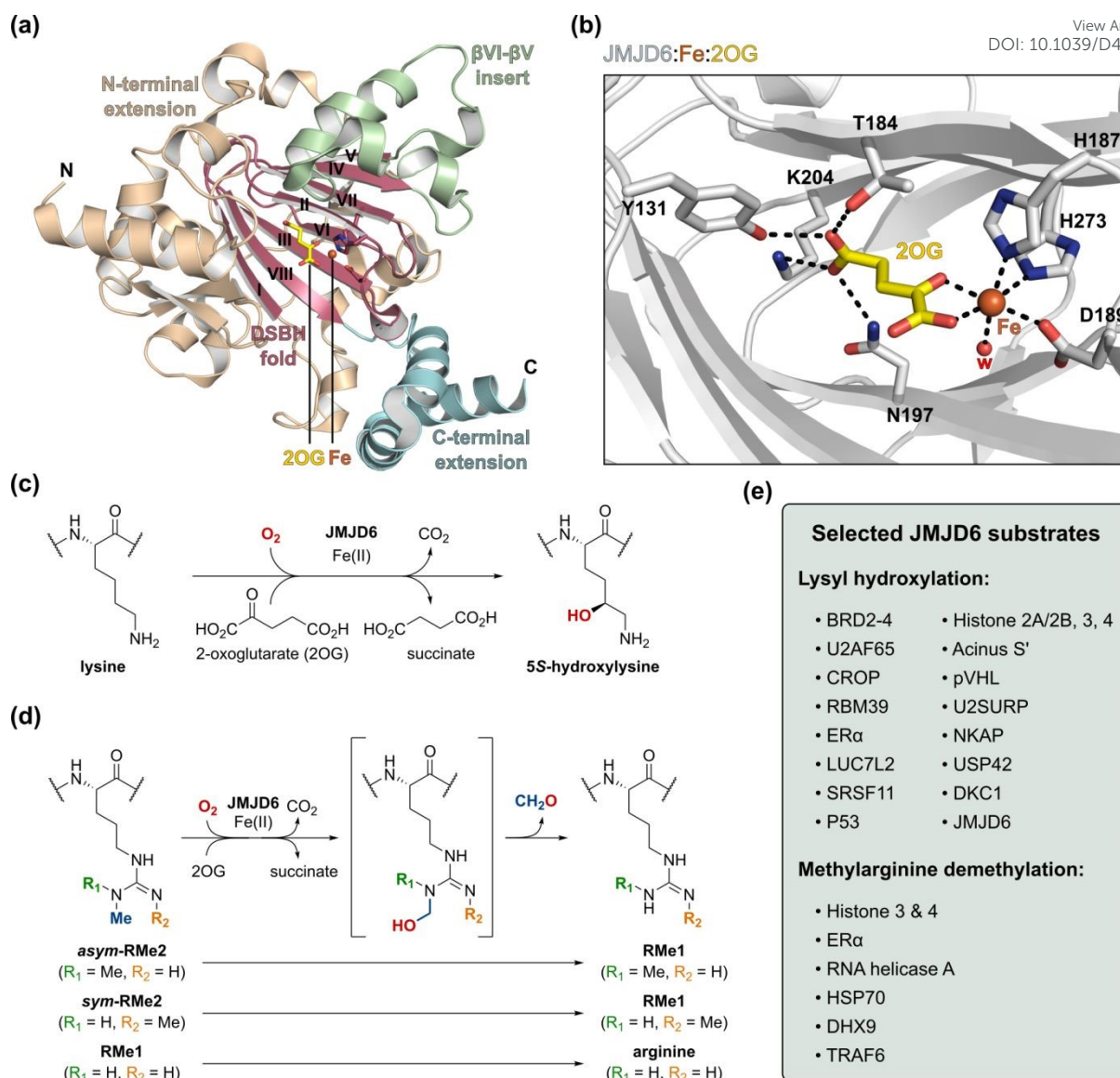
Figure 1. The human 2-oxoglutarate (2OG)- and Fe(II)-dependent oxygenase Jumonji-C domain-containing protein 6 (JMJD6).
