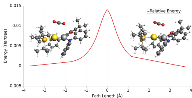
Fig. 10 One-dimensional IRC minimum energy reaction path for the first step of the reaction of the [t\text{Bu}_3\text{PAuAl}(\text{NON})] complex with \text{CO}_2 . Insets: IRC-optimized geometry for the two minima adjacent to TSI. Adapted and reprinted with permission from ref. 40 Copyright 2022, American Chemical Society.
