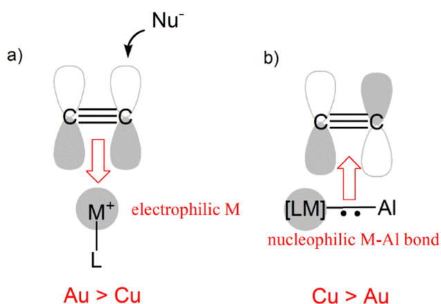
Scheme 9 (a) Electrophilic behaviour of [\text{LM}]^+ ( \text{M} = \text{Cu}, \text{Au} ) complexes for alkyne activation (Au more efficient than Cu); (b) nucleophilic behaviour of the M–Al ( \text{M} = \text{Cu}, \text{Au} ) bond in coinage metal–aluminyl complexes towards alkynes (Cu more efficient than Au).
