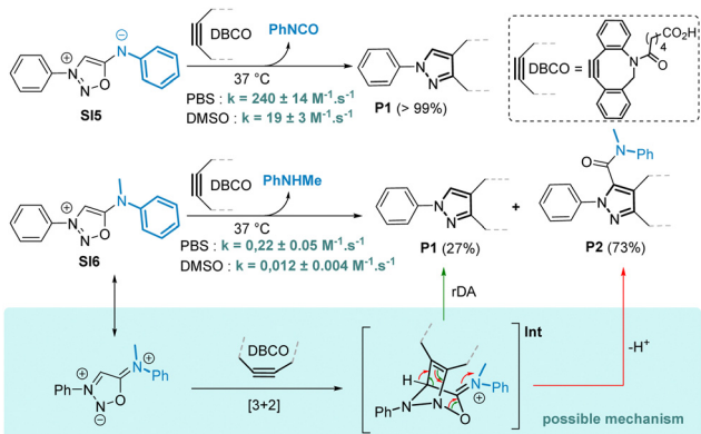
Scheme 4 Reaction of syndonimines SI5 and SI6 with DBCO. Proposed mechanism for the formation of P1 and P2 from SI6 . The rate constants were determined by UV monitoring, [\text{SI5}] = [\text{SI6}] = 100 \mu\text{M} , DBCO 1.0 equiv. in 0.1 M PBS pH = 7.4 or in DMSO. Yields of pyrazoles were estimated by ^1\text{H} NMR monitoring in DMSO- d_6 .
