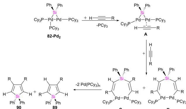
Scheme 32 Possible pathway for the formation of siloles from 82-Pd 2 and terminal alkynes.
