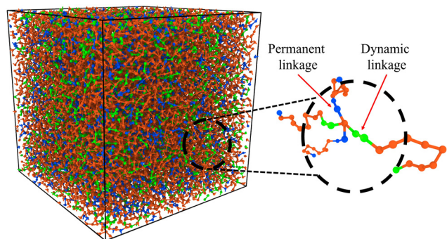
Fig. 1 Simulation box snapshot of hybrid vitrimer network. The blue beads represent the segments with permanent crosslinks, and the green beads show the dynamic linkages. The orange beads represent the linear polymer chains rendered using OVITO. 32
