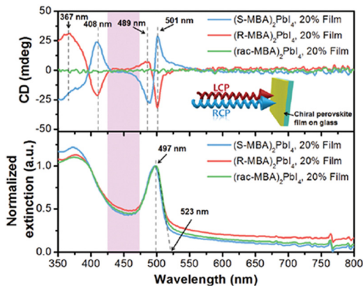
Fig. 4 Transmission CD spectra (above) and normalized extinction spectra (below) of (R/S/Rac\text{-MBA})_2\text{PbI}_4 (in the inset a pictorial representation of a HOIP thin film irradiated by LCP/RCP light). Reprinted with permission from ref. 11 Copyright©2017 Royal Society of Chemistry.
