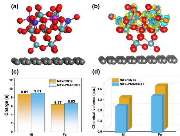
Fig. 4 (a) Optimized structures of the NiFe-PMA/CNT catalyst. The balls in grey, red, pink, blue, violet and cyan represent C, O, P, Ni, Fe and Mo atoms, respectively. (b) The 3D differential charge density of the NiFe-PMA/CNT catalyst. The green symbols represent a decrease in charge density, while the yellow symbols represent an increase in charge density. (c) The charge of Ni and Fe atoms on NiFe/CNTs and NiFe-PMA/CNTs from Bader charge analysis. (d) The chemical valence state of Ni and Fe atoms on NiFe/CNTs and NiFe-PMA/CNTs from Bader charge analysis.
