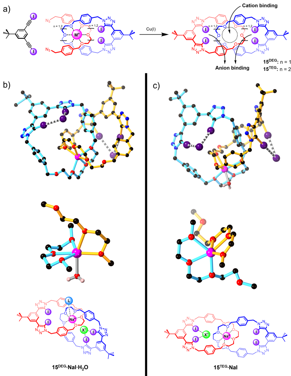
Fig. 11 (a) Sodium cation template-directed synthesis of heteroditopic all-XB [2]catenanes 15 for alkali metal halide ion-pair binding; solid-state structures of (b) 15^{\text{DEG}} \cdot \text{NaI} \cdot \text{H}_2\text{O} and (c) 15^{\text{TEG}} \cdot \text{NaI} , showing a single [2]catenane unit bound to a sodium cation and two iodide anions (top) and a truncated representation of the ethylene glycol region (middle) highlighting the coordination environment around the sodium ion. Atom colours are as follows: black (carbon), blue (nitrogen), red (oxygen), purple (iodine), light pink (hydrogen), bright pink (sodium). The chemical structures of 15^{\text{DEG}} and 15^{\text{TEG}} are shown below for reference.
