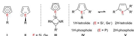
Fig. 1 Molecular structures of 1-tetrolides I and II ; planar, silylene-substituted tetrolides III and 1 H /2 H -phosphole and tetrolide rearrangements IV \rightarrow V .
