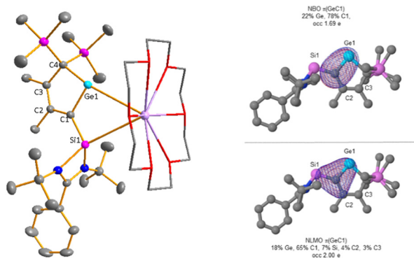
Fig. 5 Left: Molecular structure of [\text{K}(\text{18-c-6})][\mathbf{11}] in the crystal (hydrogen atoms are omitted; thermal ellipsoids at 50% probability). Selected atom distances [pm] and angles [°]: Si1–C1 183.04(2), Ge1–C1 187.39(15), Ge1–C4 207.41(2), C1–C2 144.90(27), C2–C3 136.42(26), C3–C4 150.70(22), K–Ge1 348.20(6), K–Si1 353.79(6), Si1–C1–C2 135.9, Si1–C1–Ge1 111.30(7), Ge1–C1–C2 112.74(1), C1–Ge1–C4 87.46(6). Right: Surface diagram of the NBO ( \pi(\text{GeC1}) ) and of the NLMO ( \pi(\text{GeC1}) ) showing the delocalization of the GeC1 bond (M062X/6-311+G(d,p), isosurface at 0.04).
