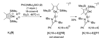
Scheme 5 Synthesis of potassium 5-silylene-2H-germol-1-ide [K(18-c-6)][11] .
