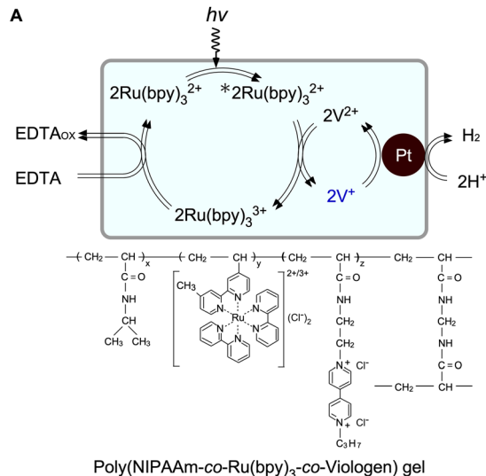
Fig. 8 (A) Photoinduced H 2 -generating system composed of a poly(NIPAAm- co -Ru(bpy) 3 - co -viologen) gel containing Pt NPs. (B) Images of the gel suspension before and after light irradiation. (C) H 2 -generation in the gel system. Reproduced from ref. 68 with permission from the Royal Society of Chemistry, Copyright 2009.
