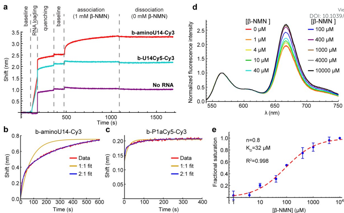
Fig. 3. (a) Bi-layer interferometry (BLI) measurements on aminoU14 (red) and U14-Cy5 RNA (cyan). Shifts are observed due to binding of RNA to the streptavidin-coated probe ("RNA loading"), binding of biocytin to the probe ("quenching") and binding of \beta -NMN to the RNA ("association"). A probe was run with no RNA loaded to control for nonspecific binding of \beta -NMN to the probe (purple). (b) Close-up of the association phase for aminoU14 RNA (red), showing fits for a 1:1 (yellow) and 2:1 (blue) \beta -NMN:RNA binding stoichiometry. (c) Close-up of the association phase for P1a-Cy5 RNA and fits. (d) Bulk FRET titration of P1a-Cy5 RNA with \beta -NMN. Emission spectra were recorded under excitation at 532 nm and the Cy3 peak was normalized to an intensity of 1. (e) Blue: titration curve extracted from the ratio of Cy5 to Cy3 emission intensity. Datapoints show the mean and standard deviation across three titrations. The curve was fit with the Hill equation (red dashed line), yielding a cooperativity of 0.8 and a K_D of 32 \mu M.
