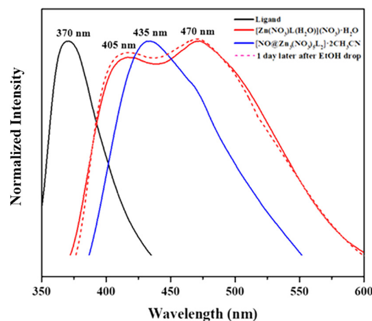
Fig. 4 PL spectra of L (black), [\text{NO}_3@Zn_3(\text{NO}_3)_5L_2] \cdot 2\text{CH}_3\text{CN} (blue), and [\text{Zn}(\text{NO}_3)\text{L}(\text{H}_2\text{O})]\text{NO}_3 \cdot \text{H}_2\text{O} (red), and transformation of [\text{NO}_3@Zn_3(\text{NO}_3)_5L_2] \cdot 2\text{CH}_3\text{CN} into [\text{Zn}(\text{NO}_3)\text{L}(\text{H}_2\text{O})]\text{NO}_3 \cdot \text{H}_2\text{O} (red dotted line).
