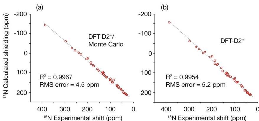
Fig. 2 A plot comparing (a) ^{15}\text{N} shift tensors obtained from the DFT-D2*/Monte Carlo ( i.e. GRANT) NMR-guided refinement method and (b) the DFT-D2* refinement method. 1
