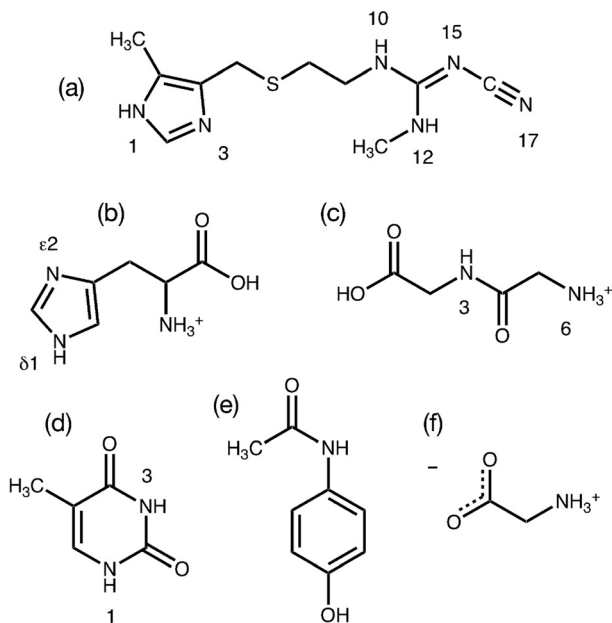
Fig. 1 Structures of the benchmark compounds studied showing nitrogen numbering. The structures evaluated include cimetidine (a), histidine HCl \text{H}_2\text{O} (b), glycyl glycine HCl \text{H}_2\text{O} (c), thymine (d), acetaminophen (e), and zwitterionic glycine (f).
