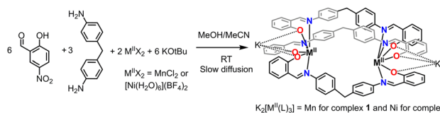
Fig. 1 Synthesis of triply stranded dianionic dimetallic helicates K_2[M_2(L)_3] , M = Mn^{2+} and Ni^{2+} , under mild reaction conditions.
